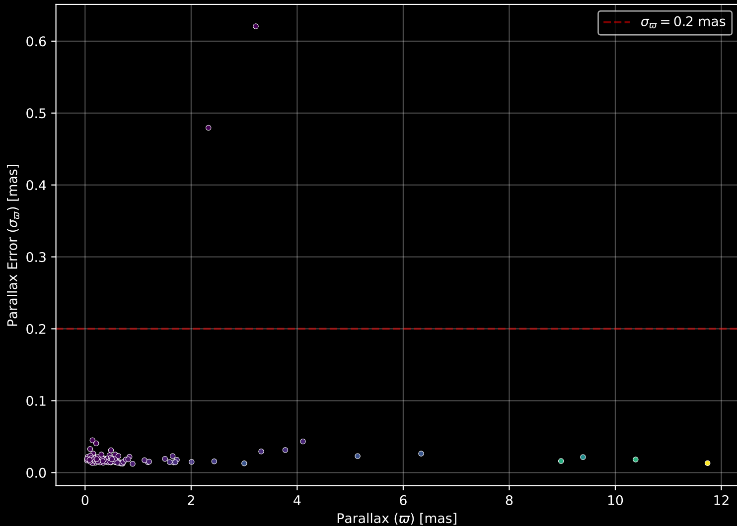
APOGEE DR17 Field: [000+16] Parallax Quality (n= 123)
