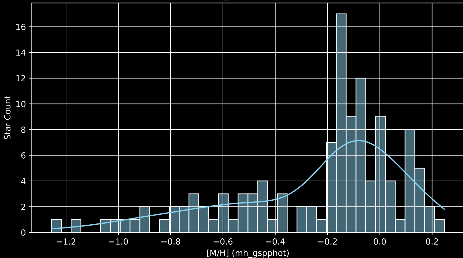
APOGEE DR17 Field: [000+16 [M/H] (mh_gspphot) (n= 121)
