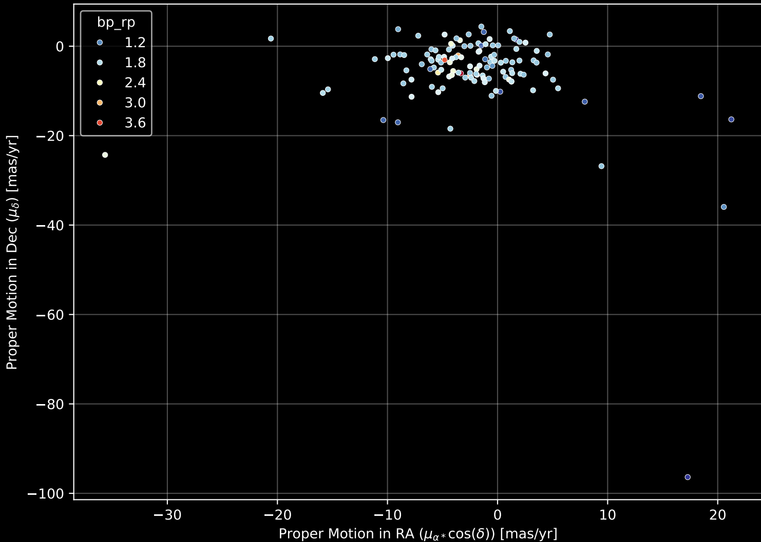
APOGEE DR17 Field: [000+16] Proper Motion Diagram (n= 123)
